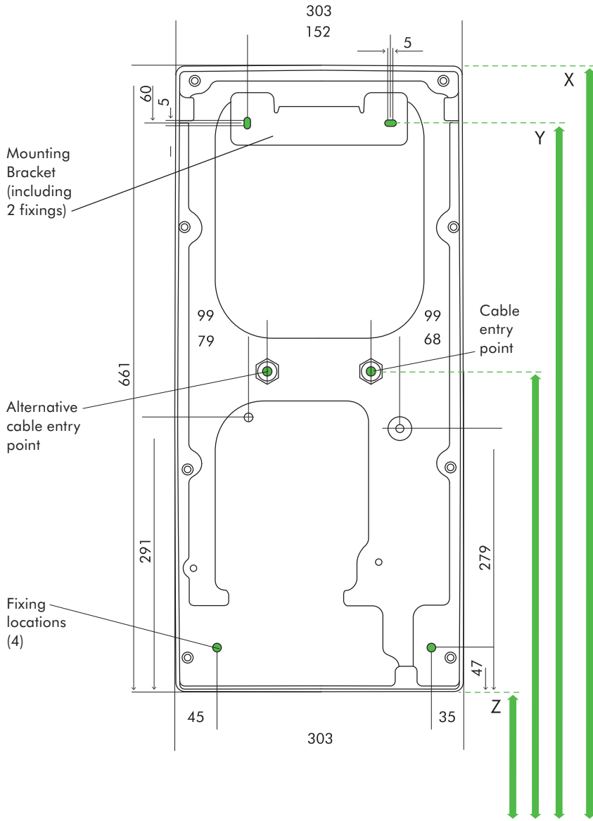
REAR ELEVATION
